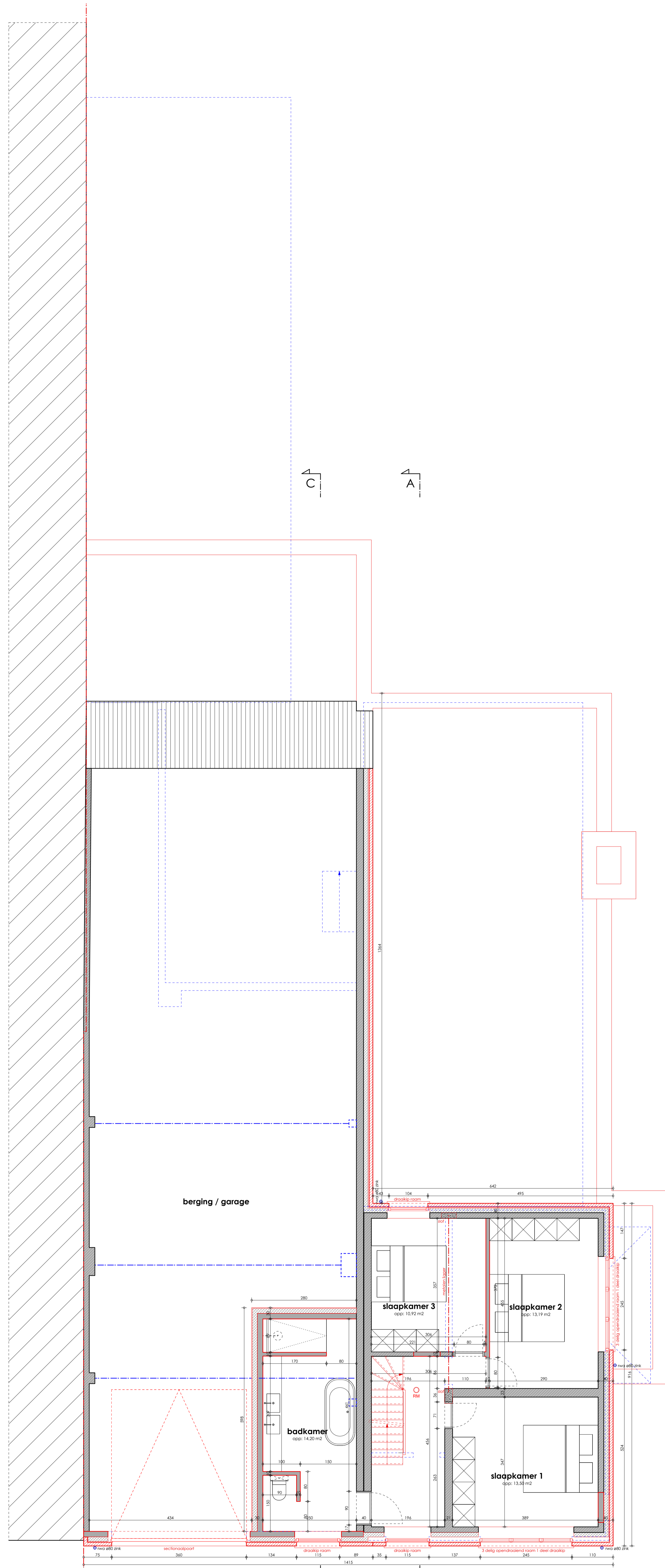
NT verdieping +1 schaal 1:50
