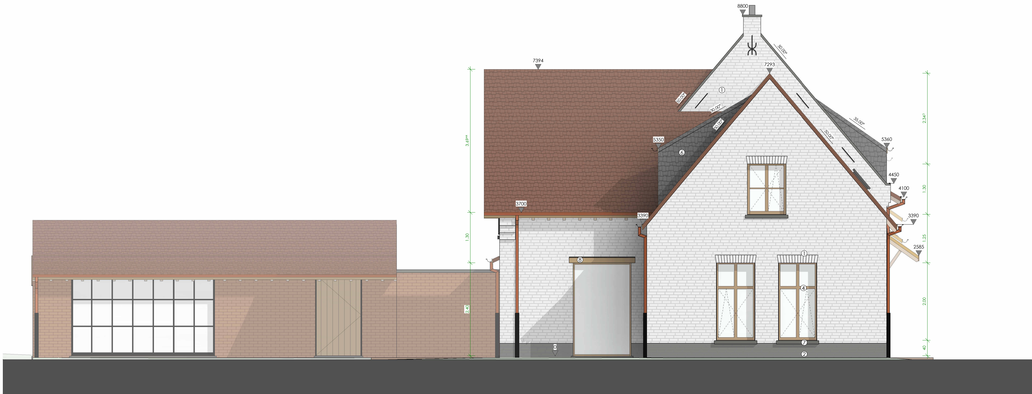
1 gevel links - BA 1 : 50 0 5m
