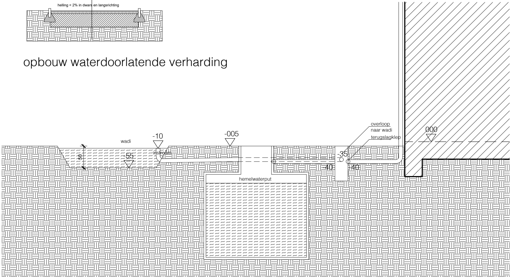
principe afloop hemelwater
